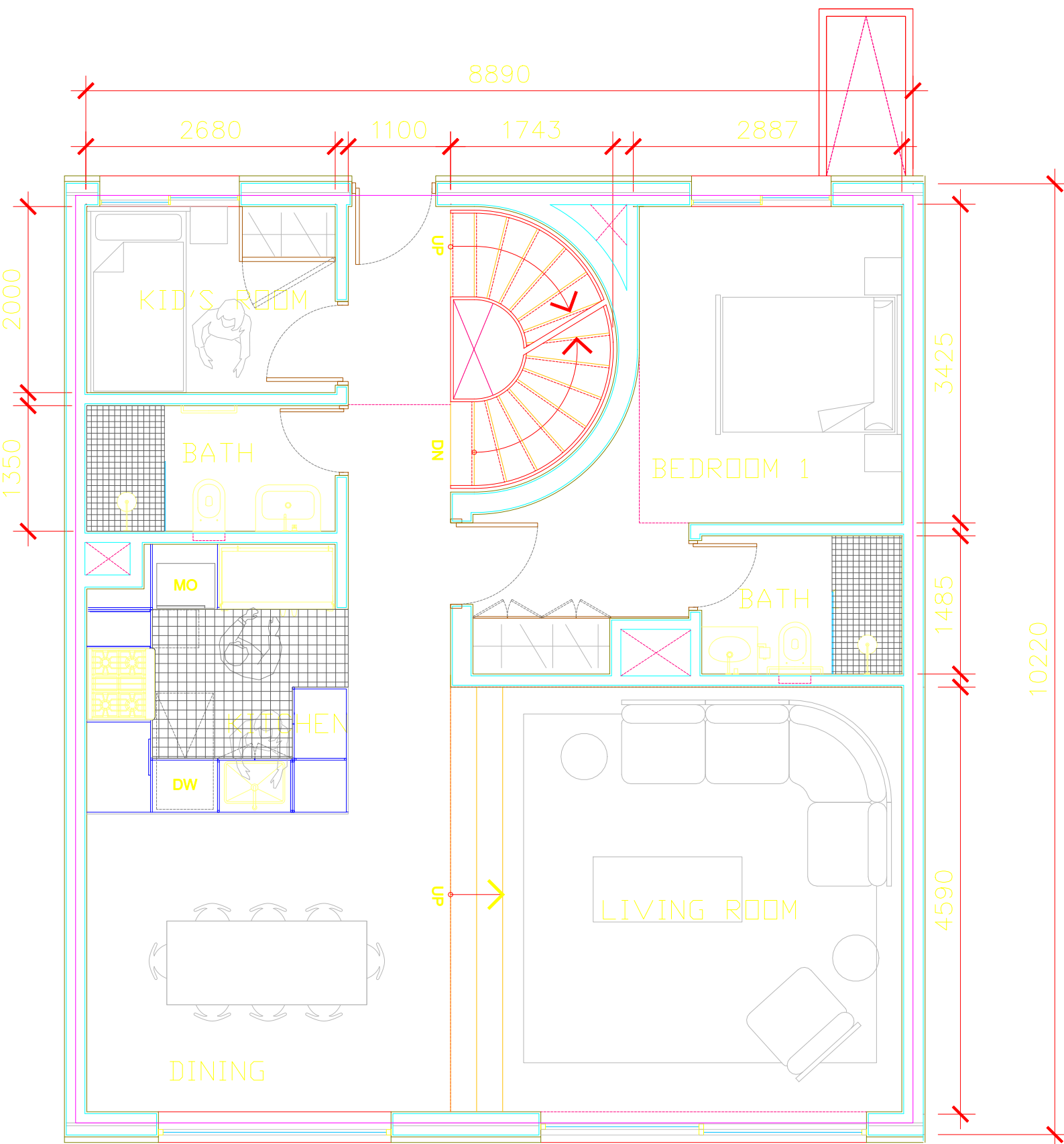
GROUND FLOOR
